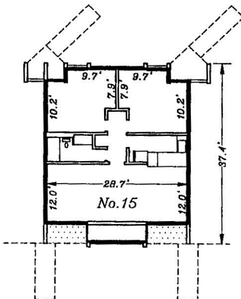
UNIT No.15 DOWNSTAIRS UNIT TYPE "C" FINISH FLOOR ELEVATION=(24.41)
