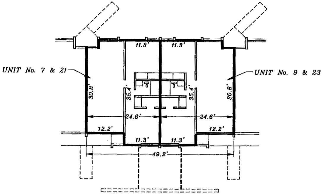
DOWNSTAIRS UNIT TYPE "B" FINISH FLOOR ELEVATION=(24.41)
