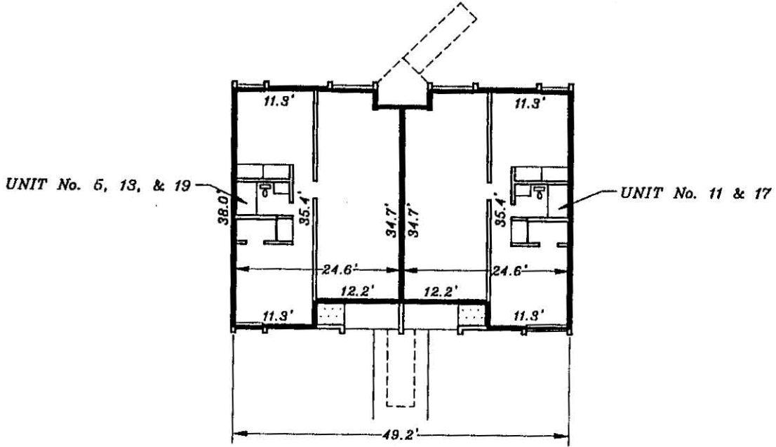
DOWNSTAIRS UNIT TYPE "A" FINISH FLOOR ELEVATION=(24.41)
