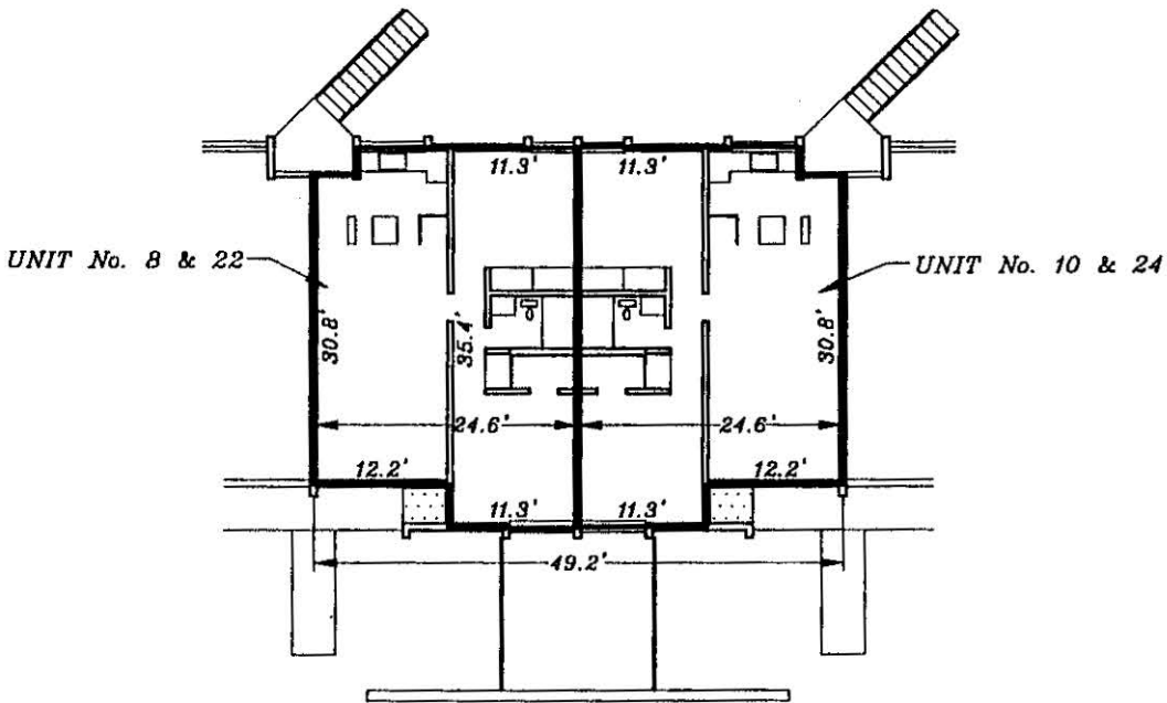
UPSTAIRS UNIT TYPE "B" FINISH FLOOR ELEVATION=(33.11)
