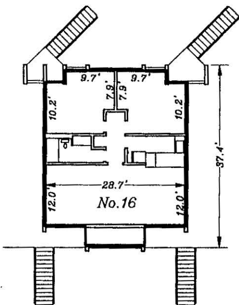
UNIT No.16 UPSTAIRS UNIT TYPE "C" FINISH FLOOR ELEVATION=(33.11)
